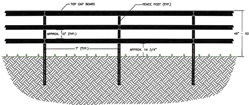
FENCING DETAIL NTS
